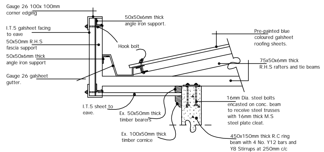
EAVE DETAIL
